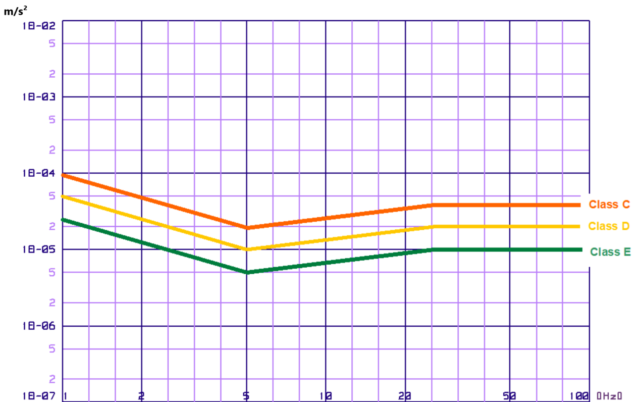
Figure 2: Vibration curves
