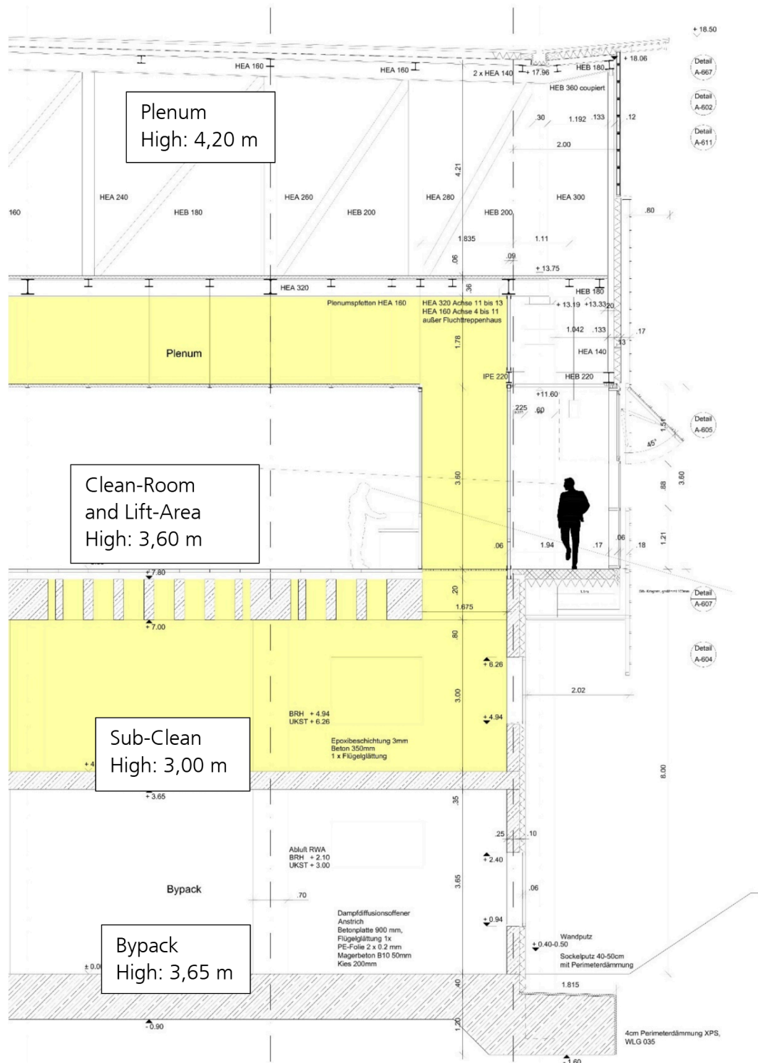
Figure 1: Fab cross-section
